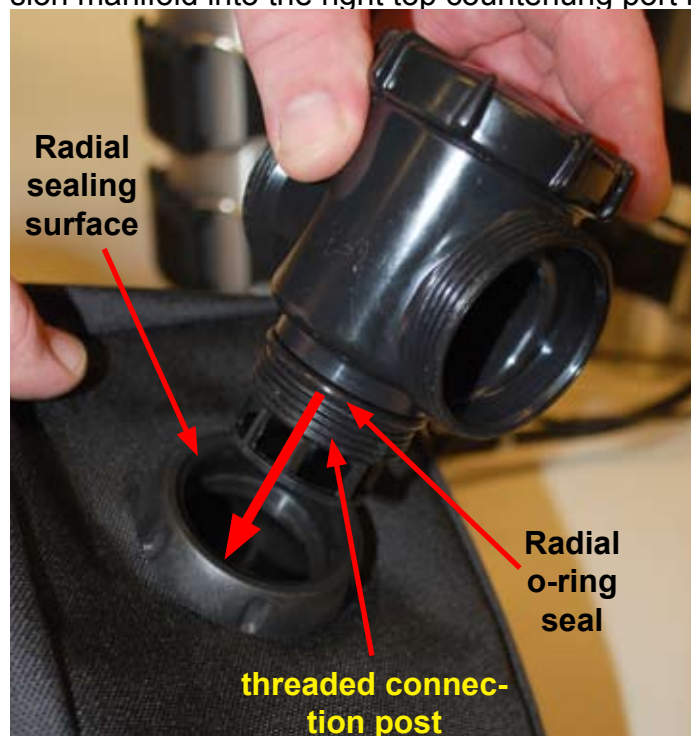
Figure 1-60. Insert the right hand water diversion manifold into the port on the right counterlung.
