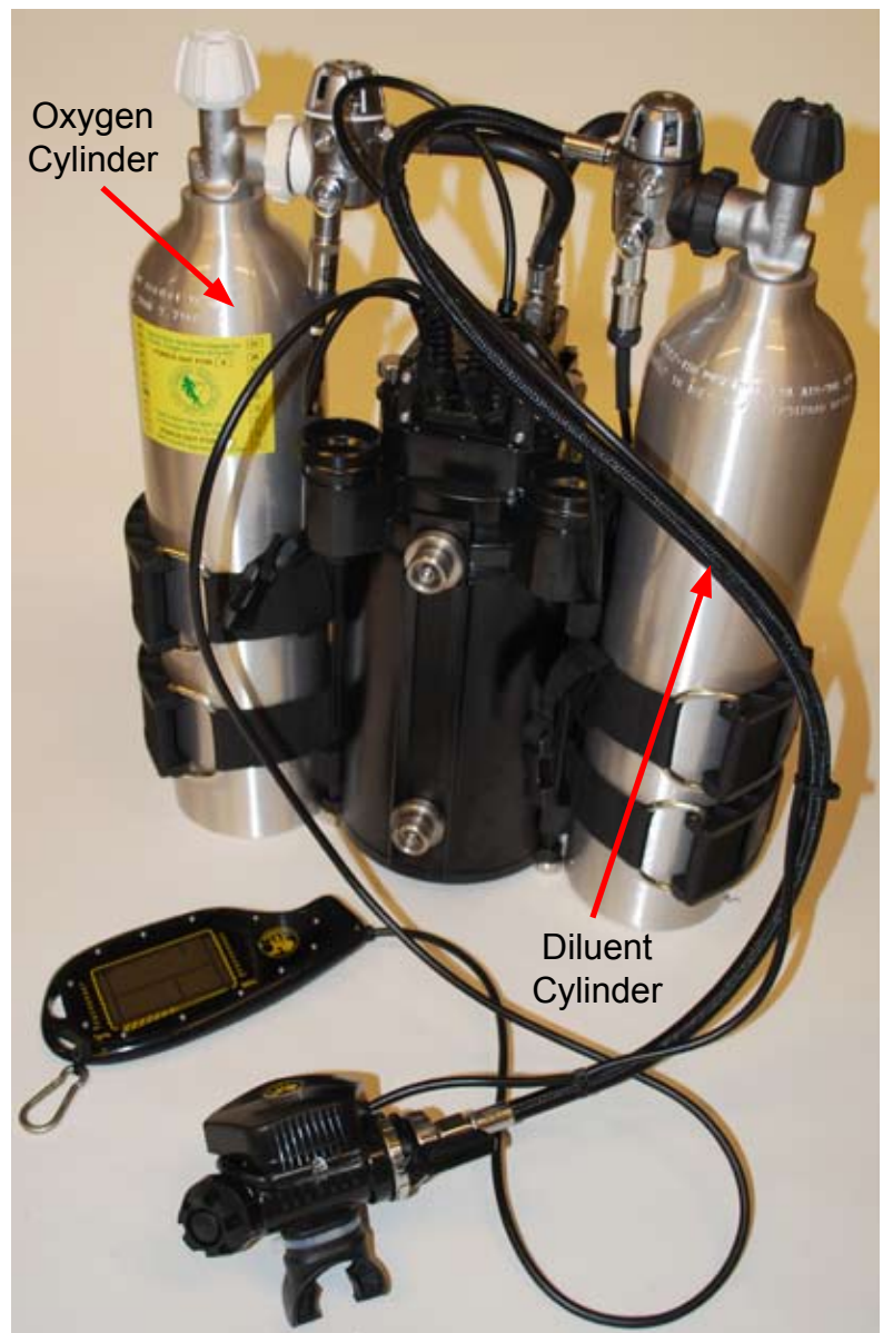
Figure 1-35. How the rig should appear when properly assembled.
