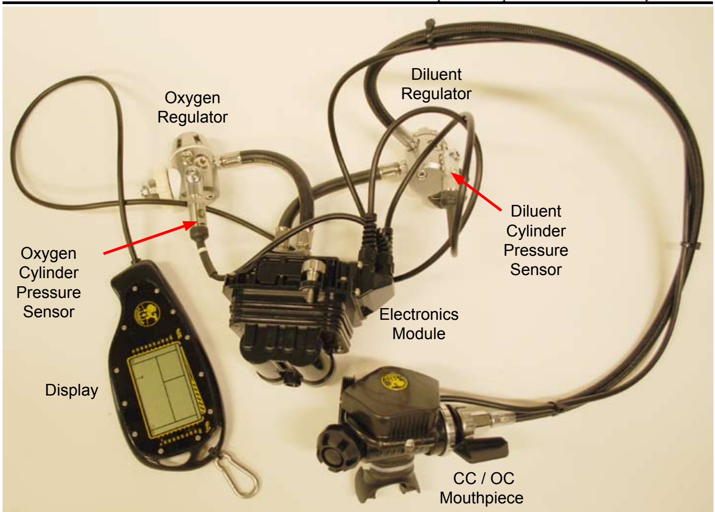
Figure 1-29. Inspect the Electronics Module and Related Components
