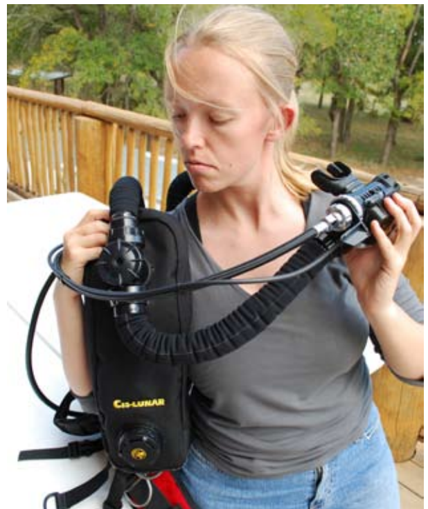
Figure 1-94. Don the harness by inserting one arm at a time through the shoulder straps.
