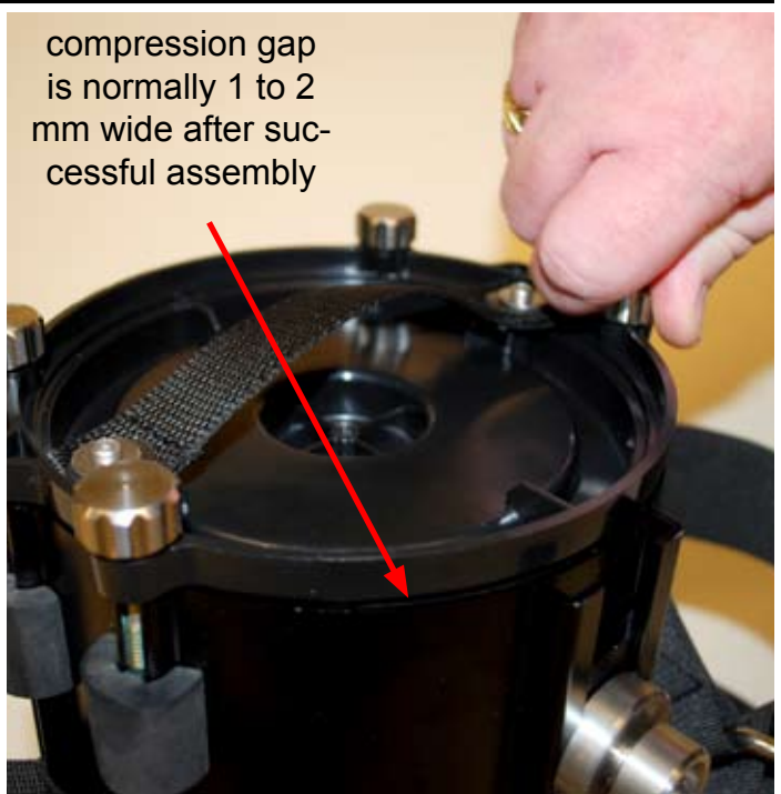
Figure 1-27. Final insertion of end cap into cartridge housing - Figure 1-28. Tighten the four hand nuts
