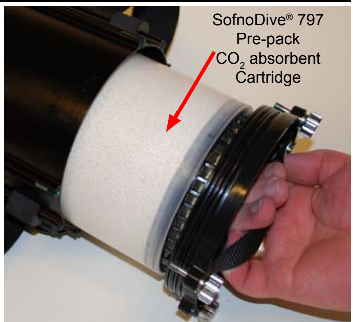
Figure 1-13. Remove the Absorbent Cartridge.
