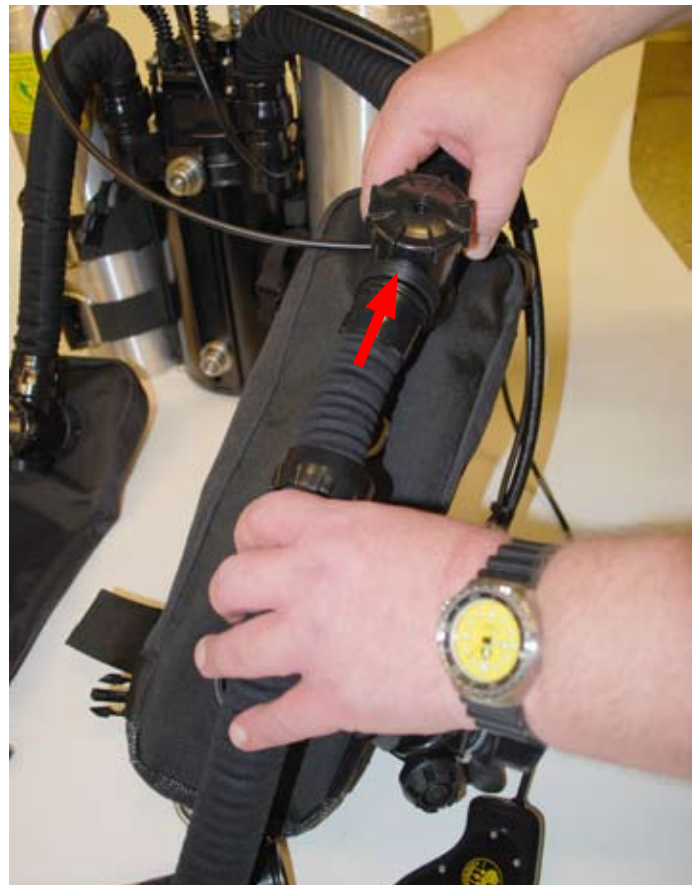
Figure 1-67. Insert the left front breathing hose into the left front shoulder port.
